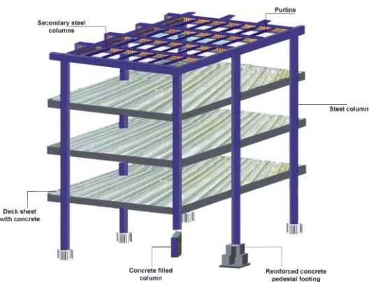
TYPICAL STEEL STRUCTURE WITH METAL DECKING SHEETS FOR MULTISTOREY & COMMERCIAL STEEL BUILDINGS
