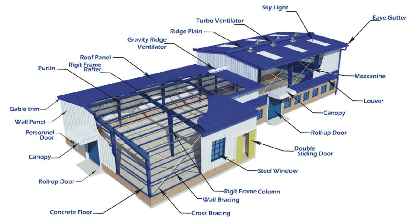
TYPICAL PRE-ENGINEERED BUILDING
